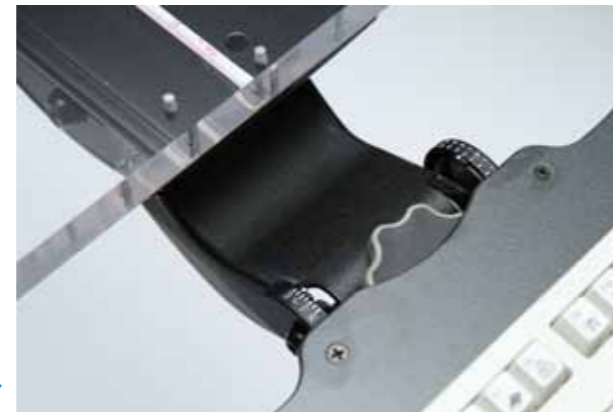
28493 Stubby EasyRiser™ Black powdercoat 14¼" Track
